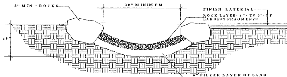
ROCK-LINED INFILTRATION TRENCH
